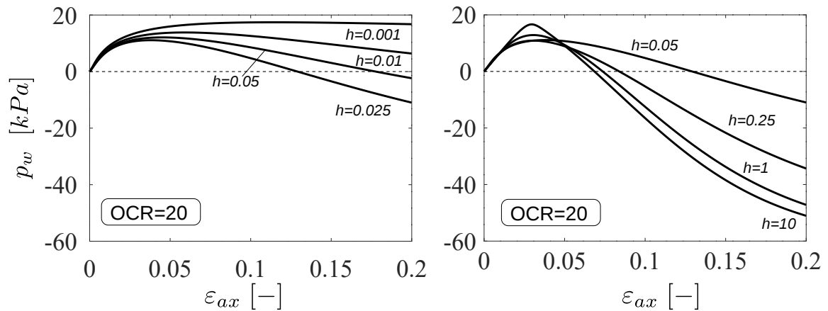
Figure 5-4: Evolution of the excess of pore pressure p_w corresponding to different values of the parameter h at the same initial over-overconsolidation ratios. The parameters listed in Table 3 to Simulate the London Clay are considered.
