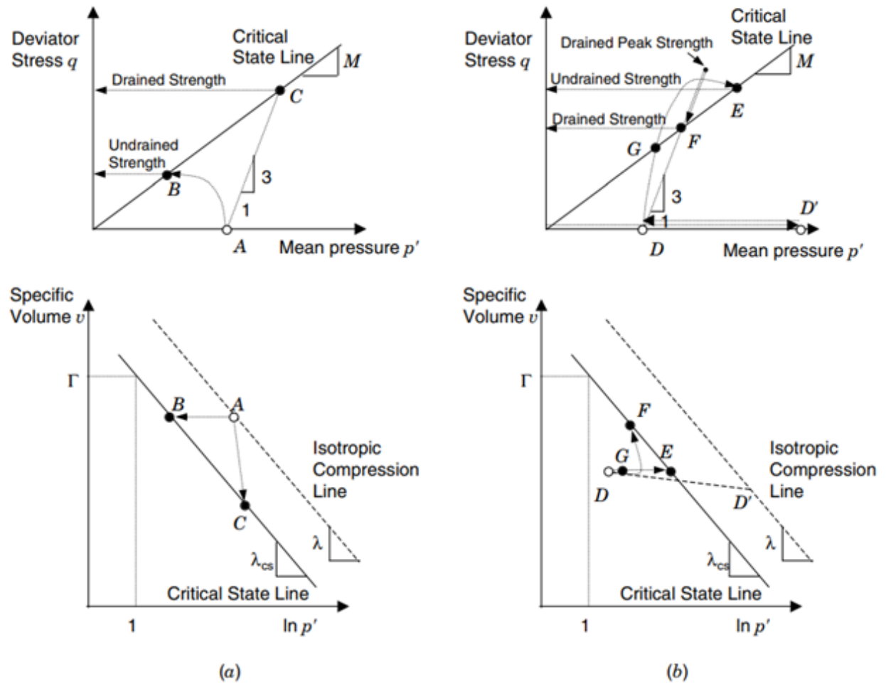
Figure 2-2: Drained and undrained stress-strain response using the critical state concept for (a) Normally Consolidated Clays and (b) Over-Consolidated Clays (figure rearranged by Mitchell and Soga, 2005)
