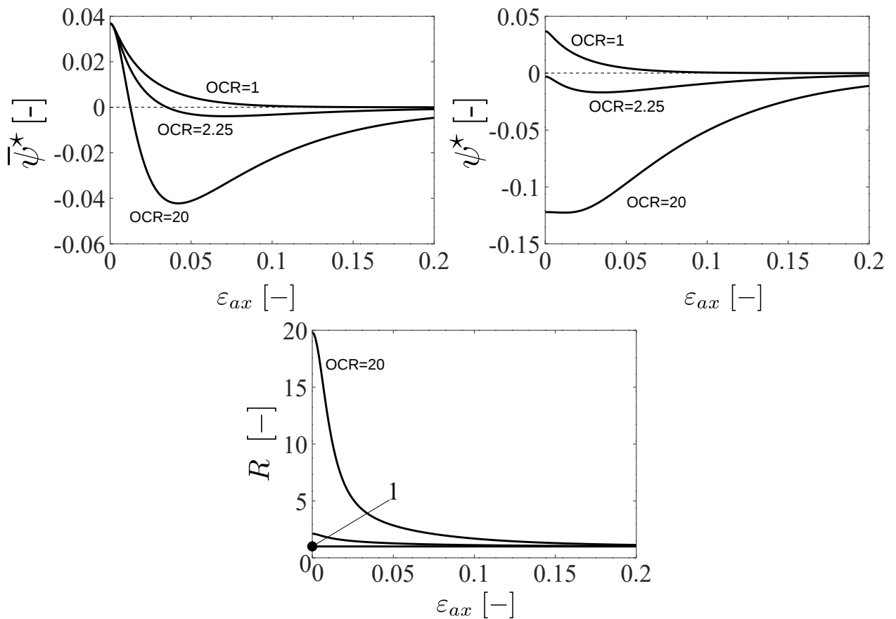
Figure 5-2: Evolution of the state parameters \psi^* , \bar{\psi}^* , and the overconsolidation ratio R during the undrained compressions reported in Figure 9
