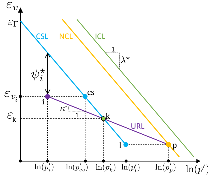
Figure 4-2: Schematic representation of isotropic consolidation line (ICL), NCL and CSL (after Wroth (1984))
