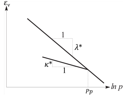
Figure 3-1: NCL and URL in \varepsilon_v - \ln(p') plane
