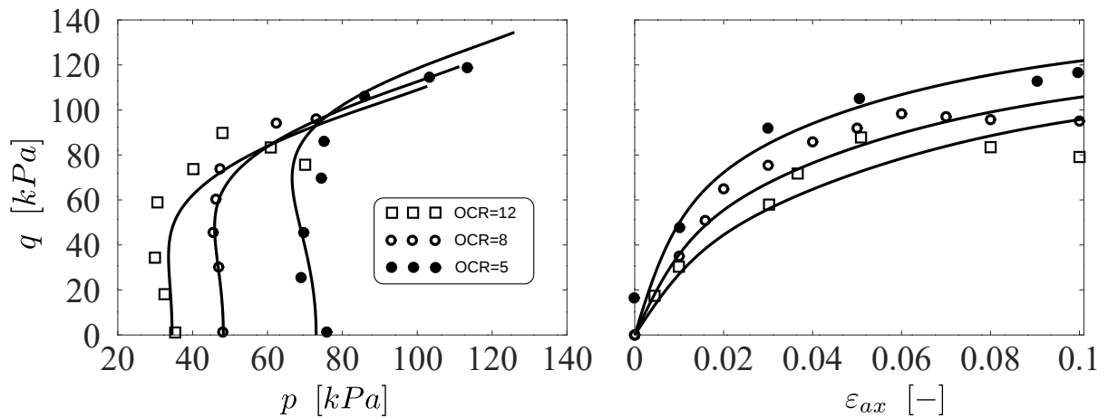
Figure 5-7: Stress paths in q - p' plane and stress-strain curves in q - \varepsilon_{ax} plane for 3 samples of Cardiff clay having different initial over-consolidation ratios
