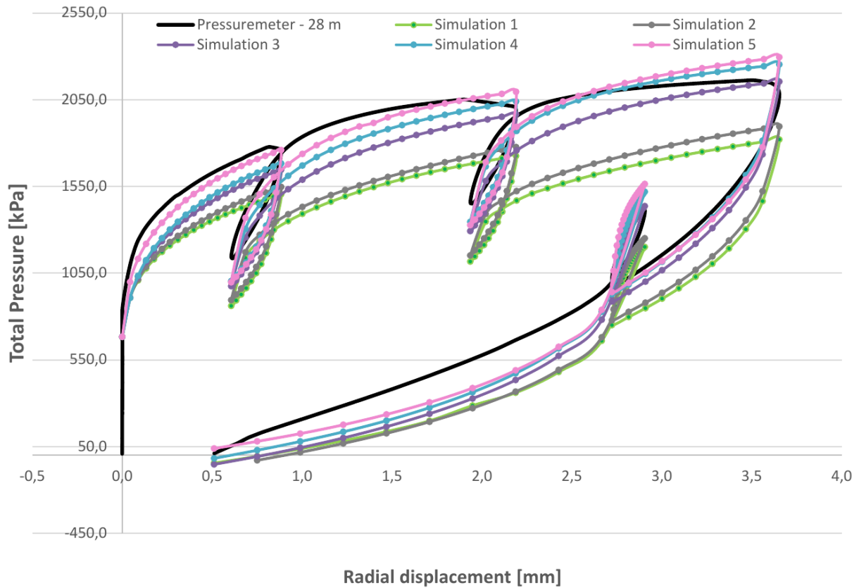
Figure 6-3: Numerical modeling of the pressuremeter test for the parameters reported in Table 15, SIM1. The pink curve corresponds to h=10 , and the parameters of the small strain model equal to G_0^{ref}=82.6 , \gamma_{0.7}=1.3 \times 10^{-4} (after Salas, 2019)
