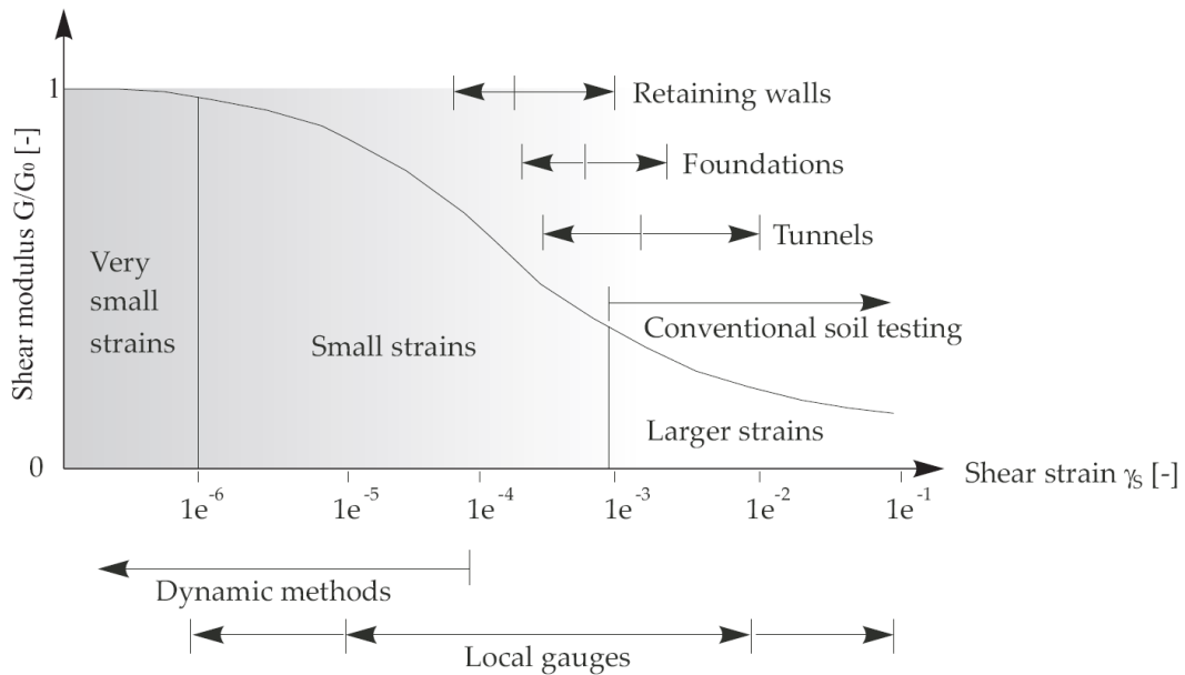
Figure 3-4: Characteristic stiffness-strain behaviour of soil with typical strain ranges for laboratory tests and structures (after Atkinson and Salfors (1991))
