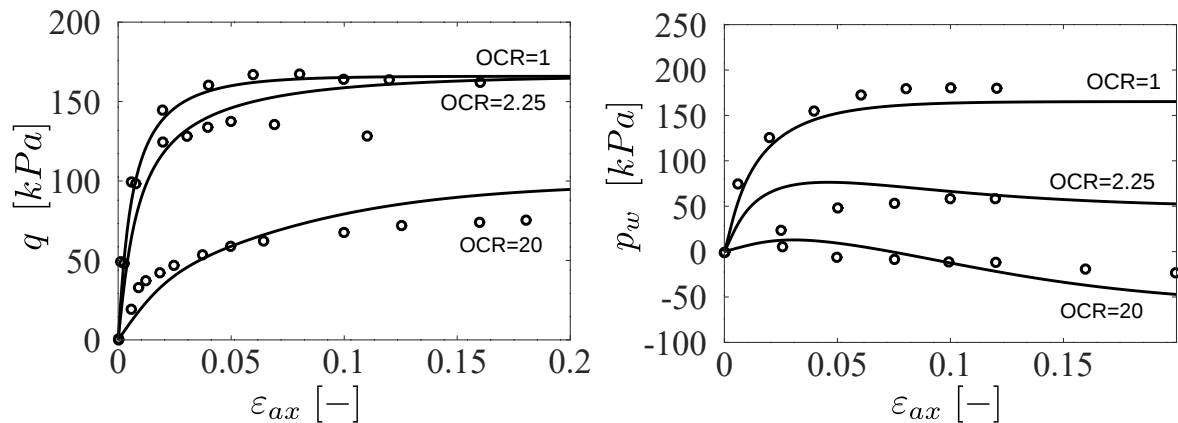
Figure 5-6: Model calibration of undrained triaxial stress paths of London Clay for different values of the over-consolidated ratio
