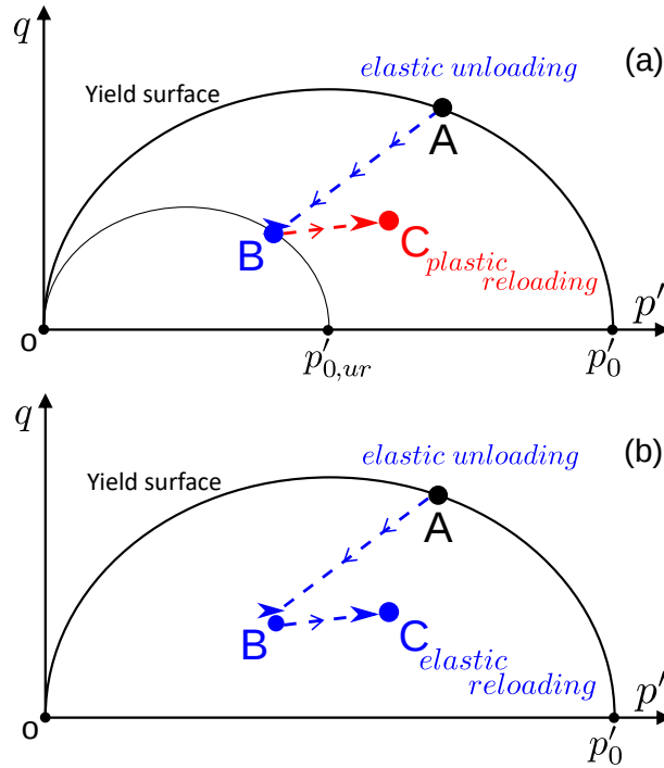
Figure 3–3: Schematic representation of the unloading behavior according to (a) the formulation of Jockovic and Vukićević (2017) (i.e., the yield surface is updated in the reloading stage, thus enabling the response in reloading to be plastic from the beginning of the loading) and (b) the elasto-plastic theory which considers the behaviour to be elastic when the stress state is within the yield surface.
