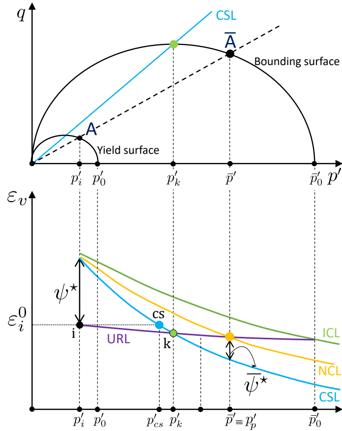
Figure 3-2: Schematic representation of the theoretical framework used in HASP model including the current stress A and its conjugate point \bar{A} (figure after Jockovic & Vukicevic, 2017)
