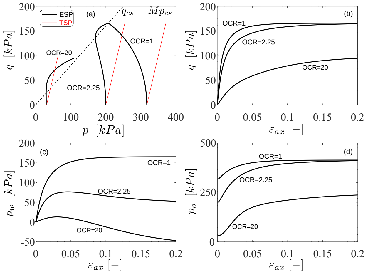
Figure 5-1: Stress paths in q - p' plane and stress-strain curves in q - \varepsilon_{ax} plane for 3 samples of London clay having different initial over-consolidation ratios
