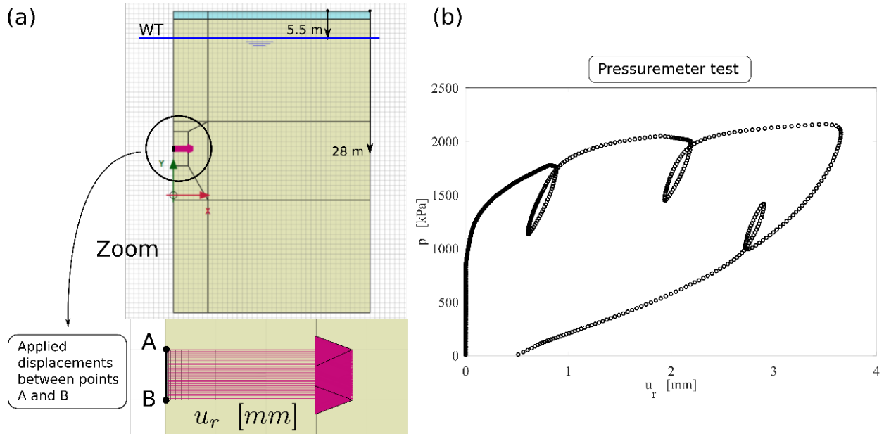
Figure 6-1: (a) Sketch of the Initial Boundary Value Problem solved to model the pressuremeter test in London Clay, (b) Experimental data after the pressure-meter test (after Salas, 2019)
