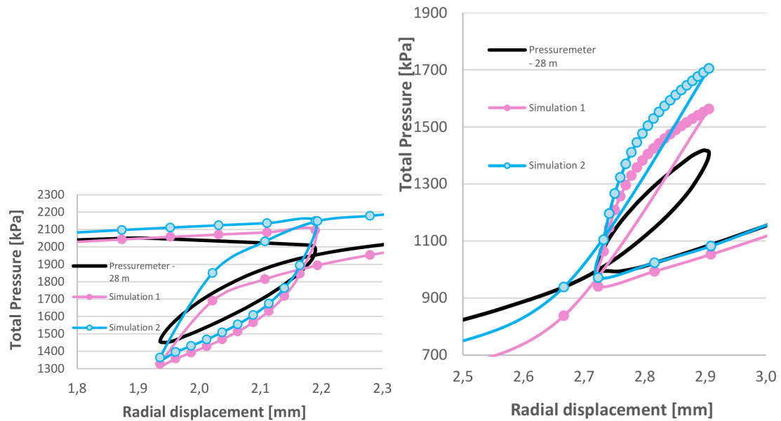
Figure 6-4: Numerical modeling for the pressure test using the parameters employed the green line in Figure 18 and by considering the different behaviour in loading and reloading (after Salas, 2019).
