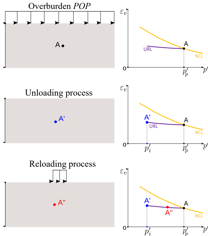
Figure 2-1: Schematic representation of the stress path resulting from an over-consolidation process
