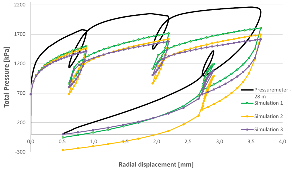
Figure 6-2: Numerical modeling of the pressuremeter for the parameters reported in Table 15 (after Salas, 2019)
