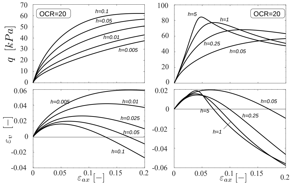
Figure 5-5: Mechanical response obtained by computing a drained stress path for different values of the parameter h
