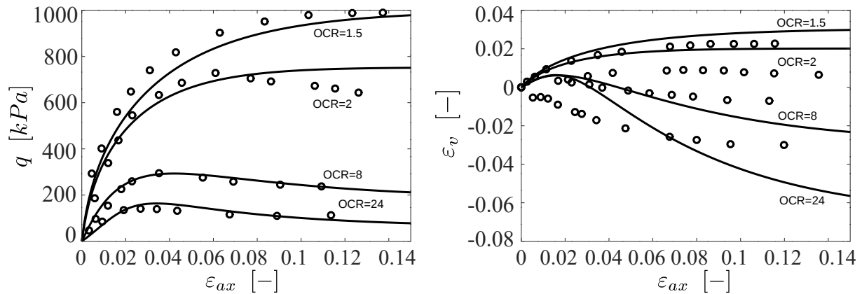
Figure 5-8: Model Calibration of Bangkok Clay by comparing the numerical results with drained triaxial tests performed are different OCR
